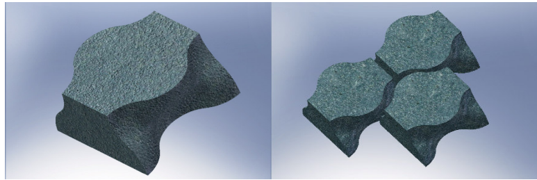
Fig. 1. Topological interlocking with osteomorphic blocks [12].
